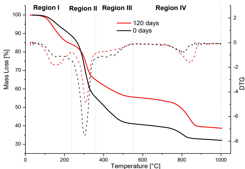
Figure 2. Comparison between POREM samples TGA and DTG at t_0 and t_{final}=120 : thermal stability and decomposition phases
