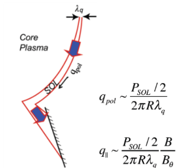
Figure 4. How to cope with large values of the power flux on the divertor: geometry helps, but by itself is not sufficient to handle a heat flux, expected to be higher than that on the sun surface.
