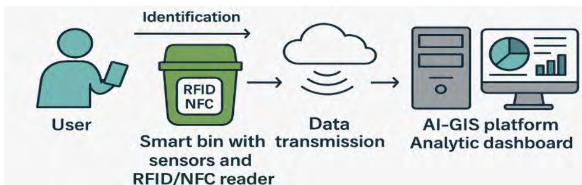
Figure 2. Data flow.
